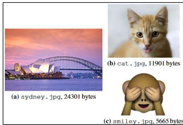
Fig. 9: Goldman's DNA stored image files [2]
