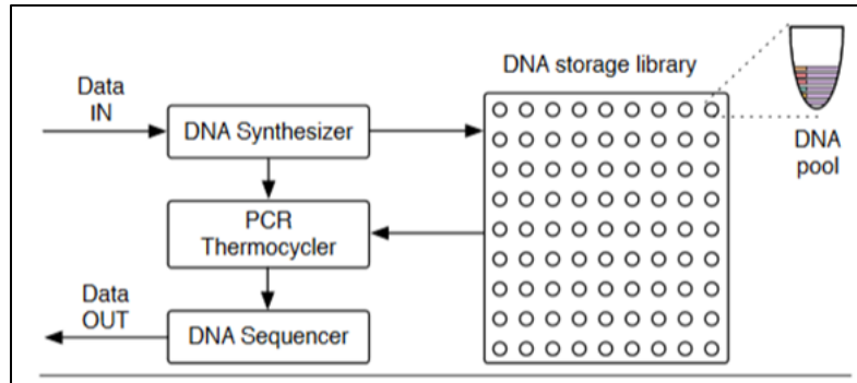
Fig. 2: The Basic Overview [6]
